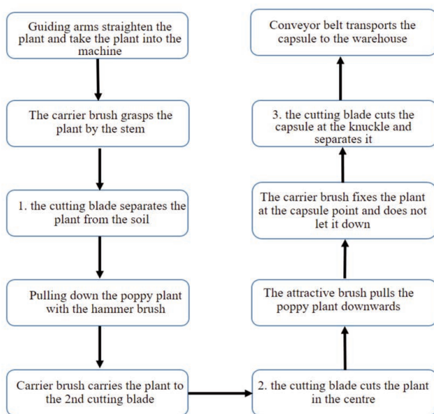
Figure 1. Workflow chart of the prototype machine.
