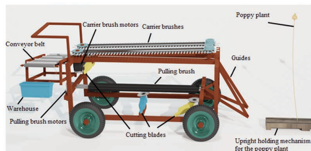
Figure 9. Solid model side view of the prototype poppy harvesting machine showing the carrier and pulling brush systems, cutting blades, and conveying mechanism.
