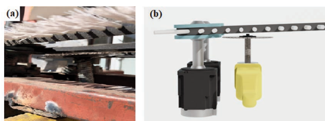
Figure 6. Cutter blade layout: realized assembly (a) and solid model view (b).
