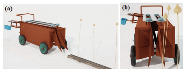
Figure 2. Prototype machine closed schematic solid model. a) Perspective view. b) Front view.
