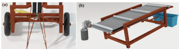
Figure 7. Additional designs: guiding arms (a) and conveyor belt (b).
