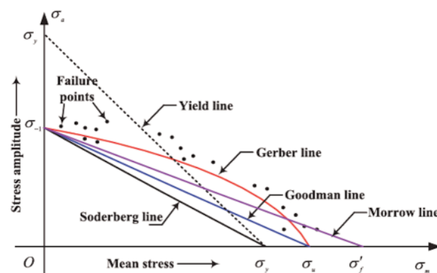
Figure 4. Mean stress correction equations for fatigue life evaluation. Retrieved from: Zhu et al. Int J Damage Mech 2017;26:1219-1241; with permission.
