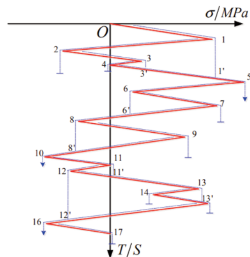
Figure 3. Operation of rainflow counting method. Retrieved from: Chen et al. Sens Transducers 2014;171:78-85; with permission.
