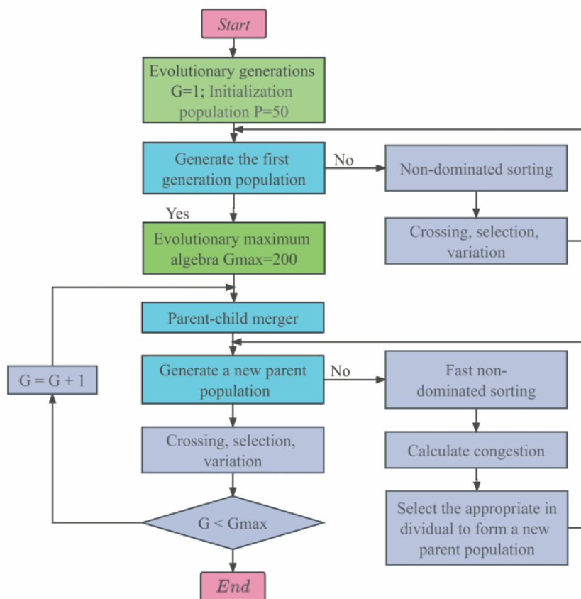
Figure 5. NSGA-II algorithm flow chart.
