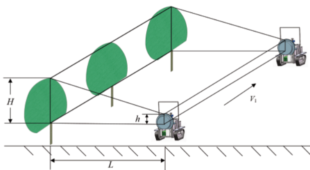
Figure 7. Schematic of air displacement principle.
