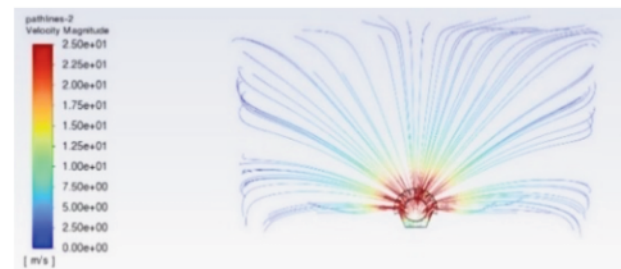
(a) deflector plate angle = 0^\circ
