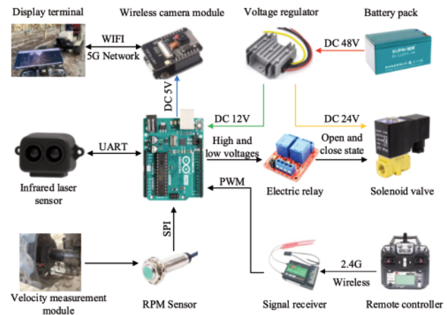
Figure 8. Hardware structure of the automatic target spraying control system.
