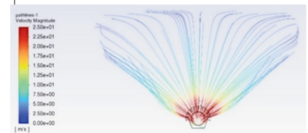
(c) deflector plate angle = 20^\circ
