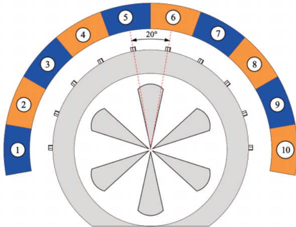
Figure 2. Schematic of nozzle arrangement.
