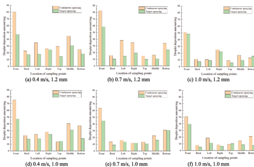
Figure 13. Droplet deposition amounts on the opposite surfaces at seven sampling points.
