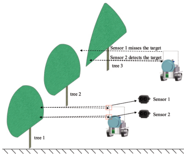
Figure 6. Schematic of infrared laser sensor arrangement.
