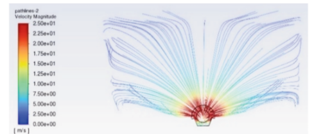
(b) deflector plate angle = 10^\circ
