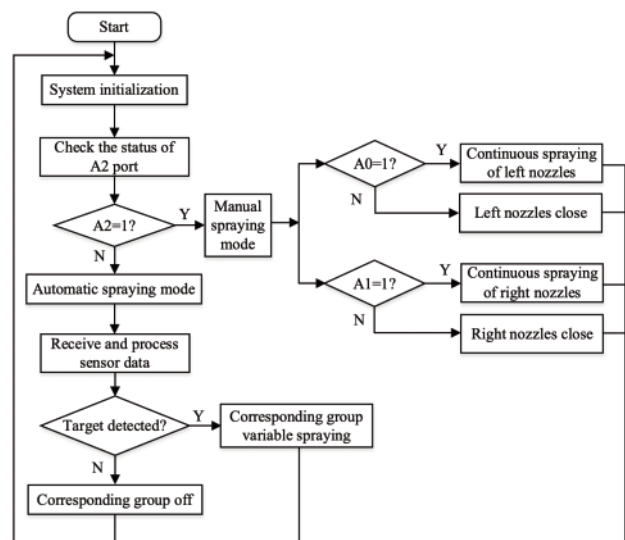
Figure 9. Control program flowchart.
