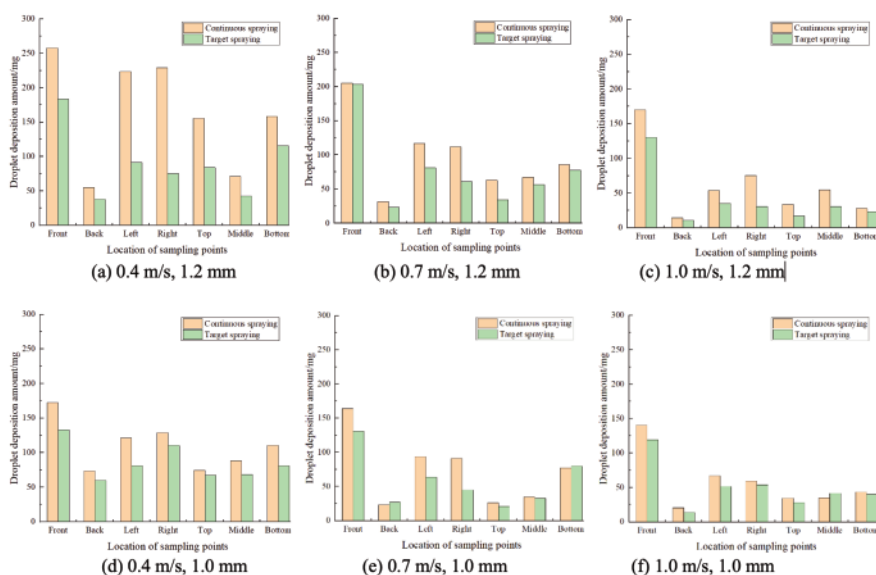
Figure 12. Droplet deposition amounts on the front surfaces at seven sampling points.
