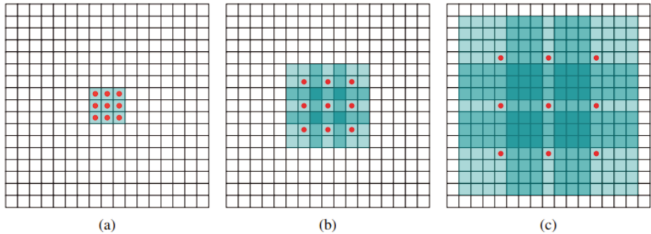
Figure 7. Extended convolution.
