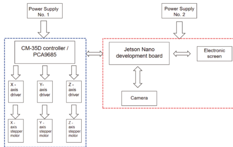
Figure 5. Structure diagram of hardware system.
