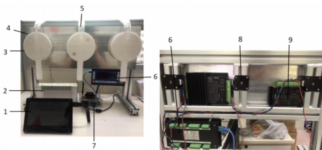
Figure 8. Experiment table of seed posture detection and adjustment device for garlic. 1, Display screen; 2, power supply; 3, turning device; 4, shell; 5, transparent conveyor pipe; 6, CM35D-40 controller; 7, Jetson Nano; 8, 42 stepper motor; 9, stepper motor controller.
