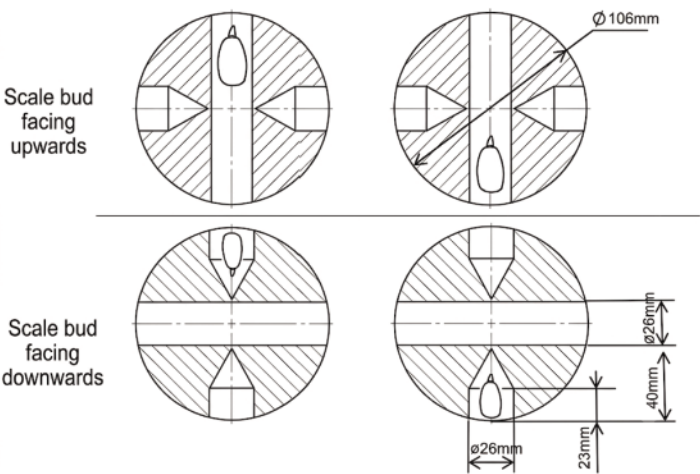
Figure 4. Working principle of garlic bud rotating plate.
