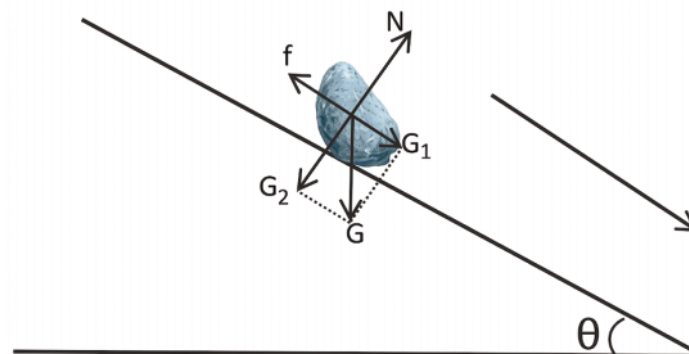
Figure 2. Force analysis of garlic seed in conveyor pipe. N , support force exerted on the garlic seed; G , gravity acting on the garlic seed; G_1 , component force of gravity acting on the garlic seed along the direction of the inclined surface; G_2 , gravity acting on the garlic seed perpendicular to the inclined plane; f , friction of the garlic seed.
