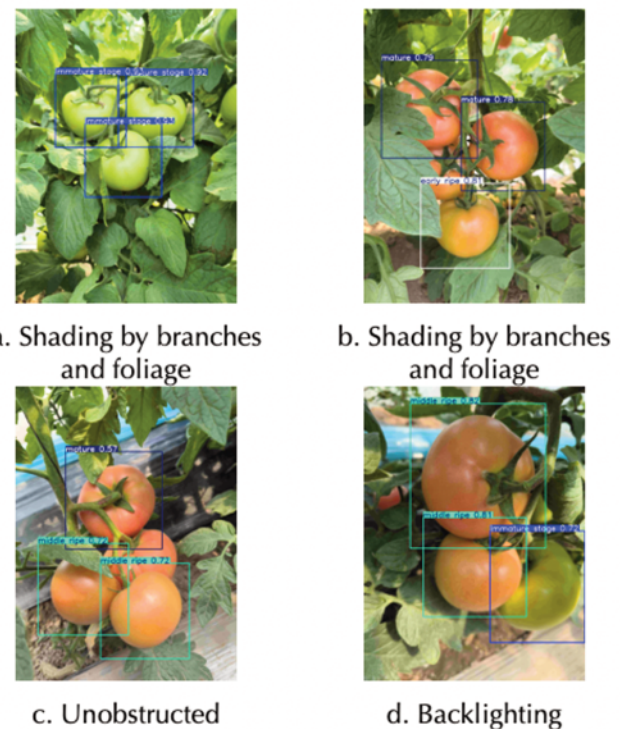
Figure 5. Improved YOLOv8 model detection results.
