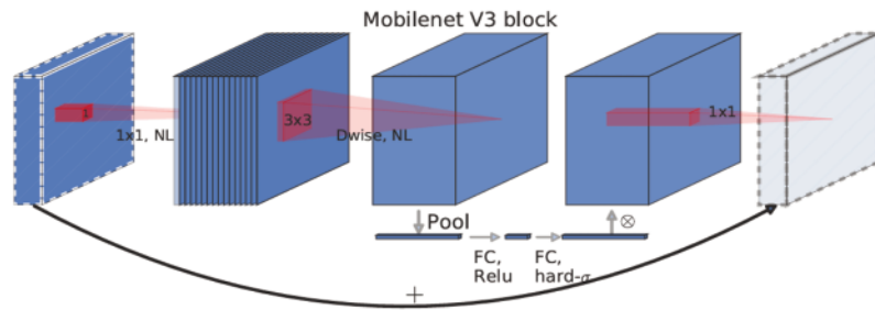
Figure 3. The bneck structure in MobileNetV3.
