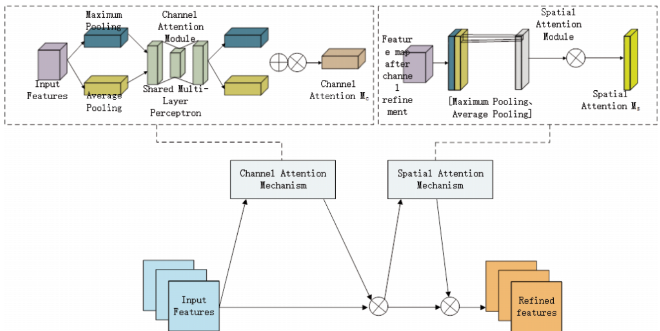
Figure 4. Convolutional attention mechanism module.
